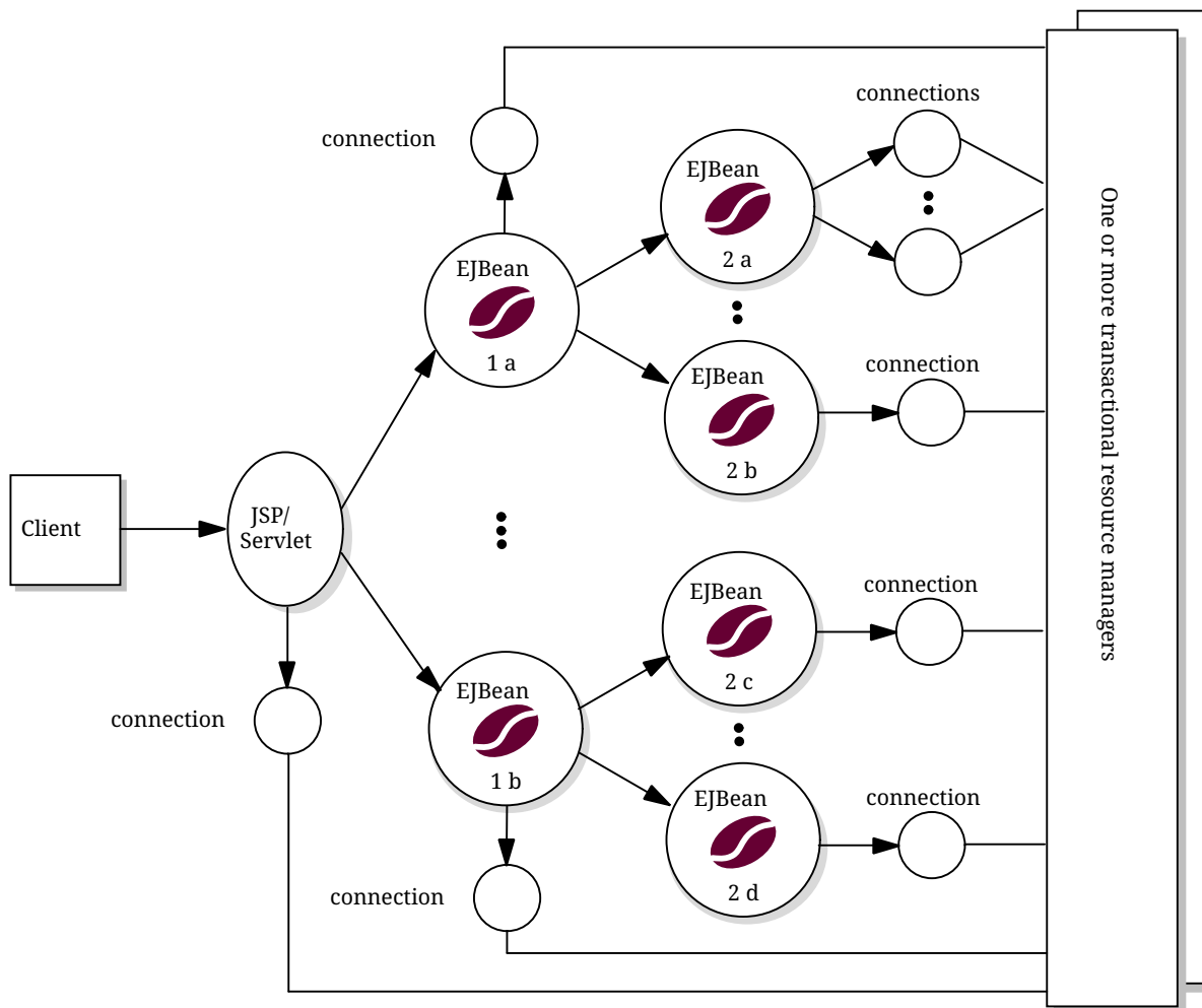
Figure 8. Servlets/Server Pages Accessing Enterprise Beans
